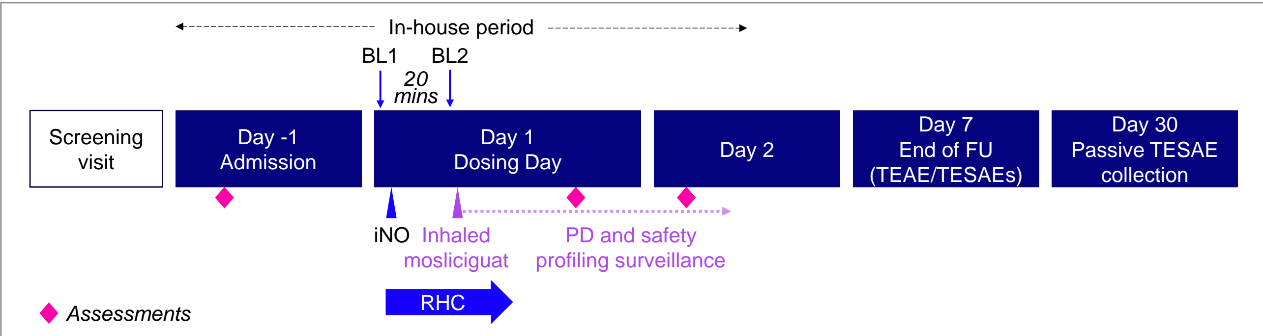
Figure 2. Study Design 12
